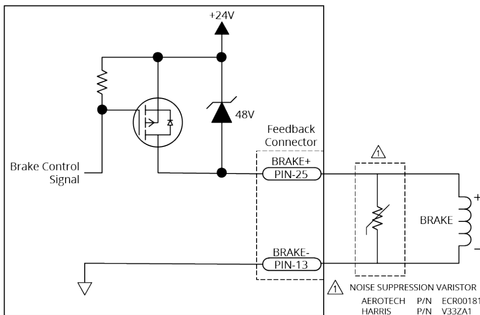
Figure 2-26: Brake Output Connections (Feedback Connector)
