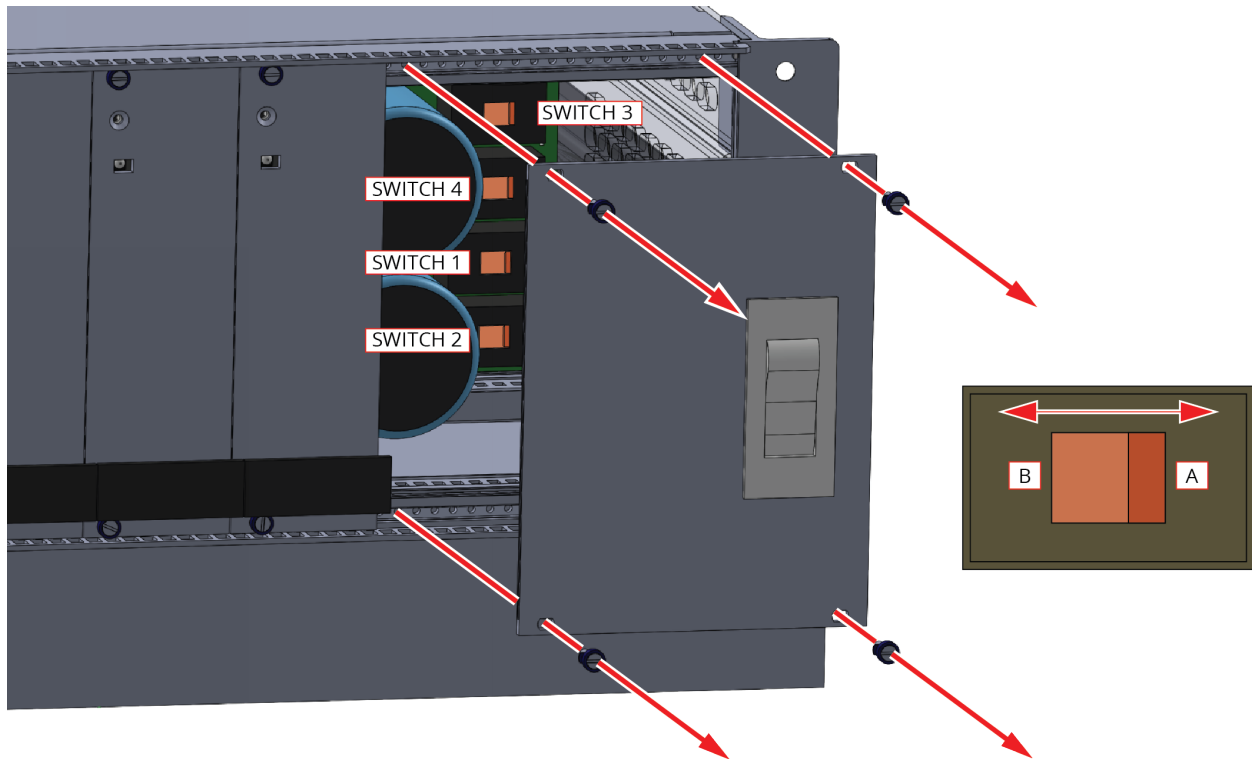
Figure B-1: Voltage Selection Switch Access
