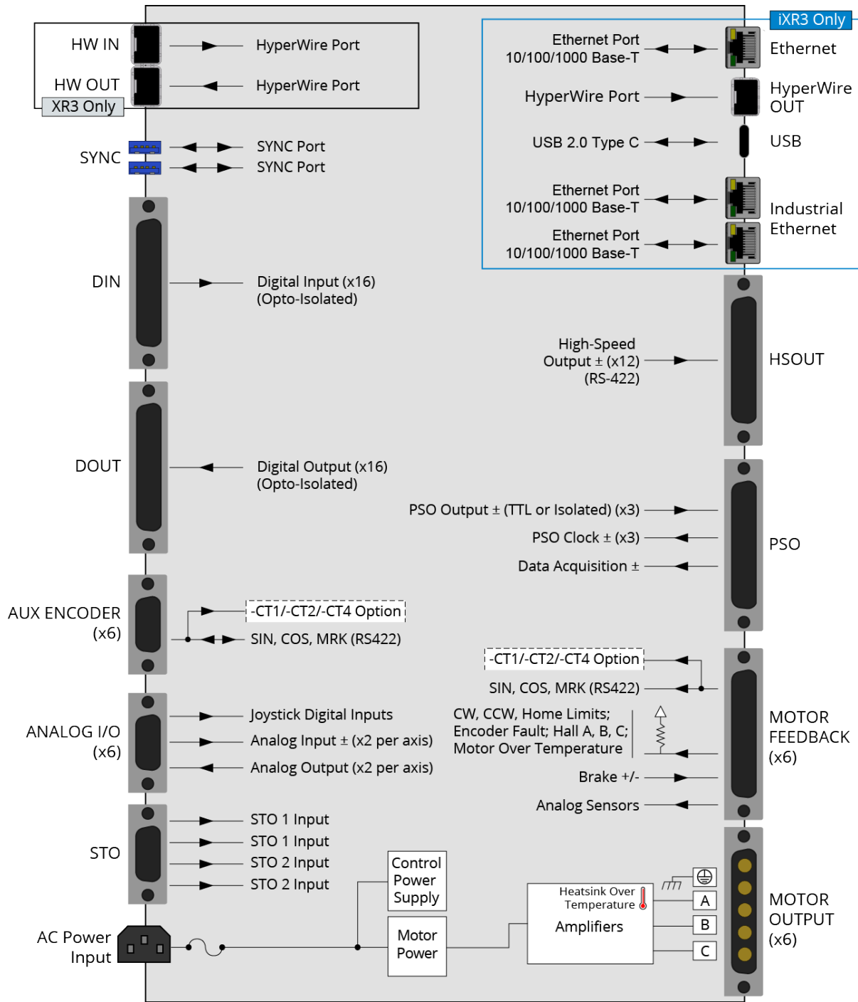
Figure 1-3: Functional Diagram
