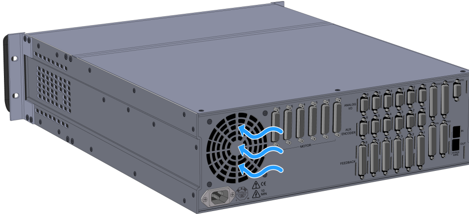
Figure 2-49: Location of the Rear Fan and Air Flow
