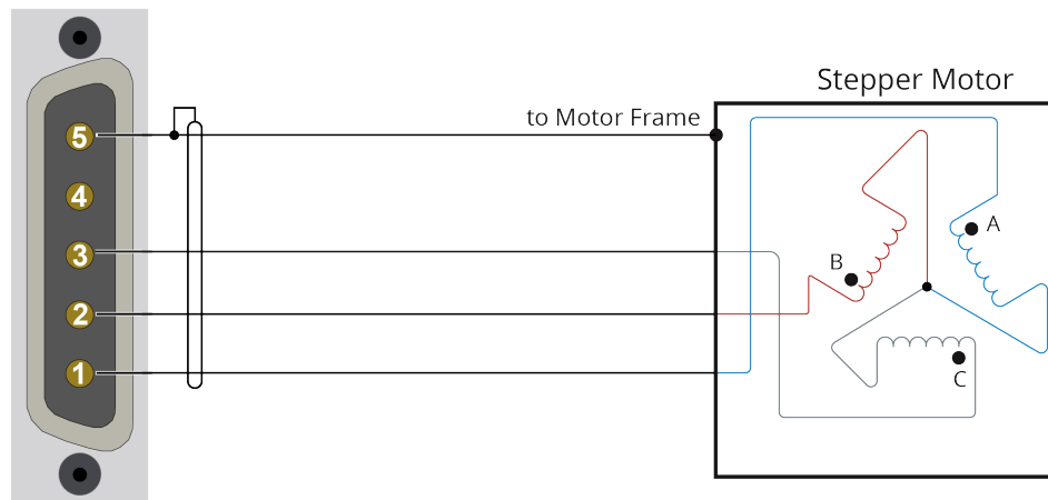
Figure 2-12: Three Phase Stepper Motor Configuration
