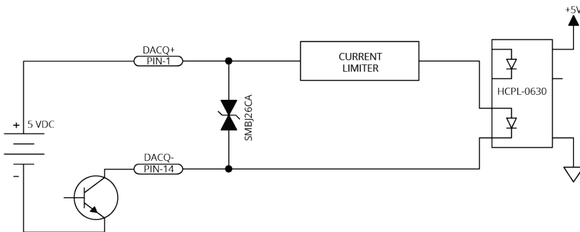
Figure 2-31: Data Acquisition Input Schematic
