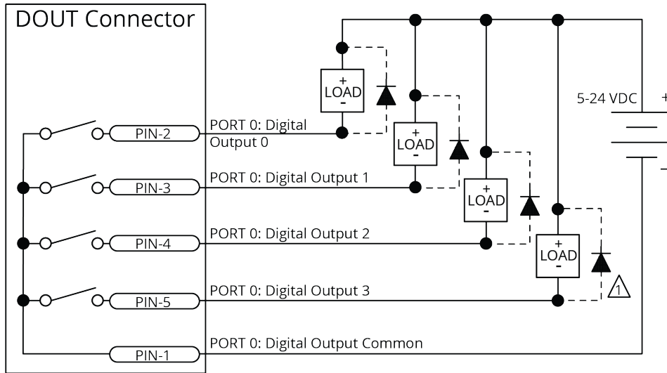
Figure 2-35: Outputs Connected in Current Sinking Mode
