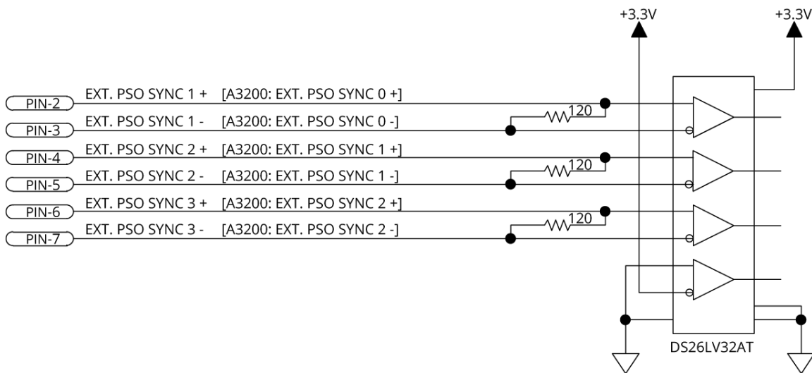
Figure 2-30: PSO Clock Inputs Schematic
