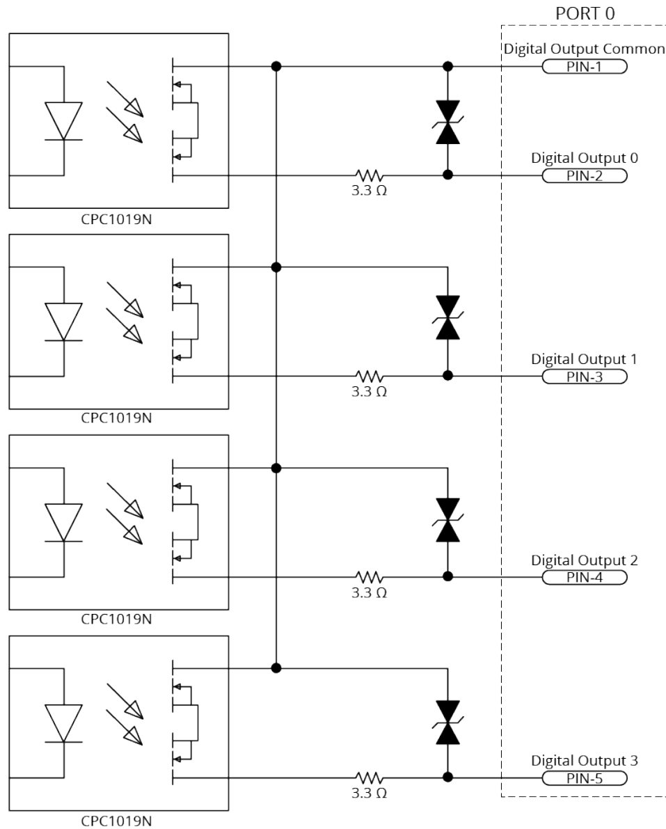
Figure 2-33: Digital Output Schematic
